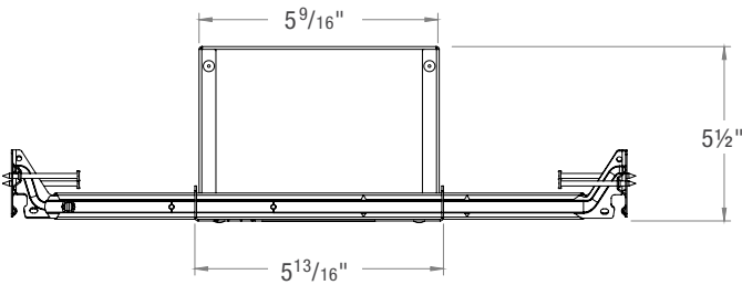
1" DOWNLIGHT, FOAM BOX ENCLOSURE
